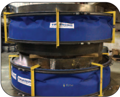
Flexi-Duct™ with K12 GSM for the Vale Clean AER Project Sudbury Canada
