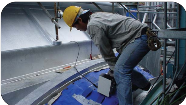
Thorburn Malaysian site team providing training on the proper procedures of splicing a KLF GSM at Malaysian gas fired power plant
