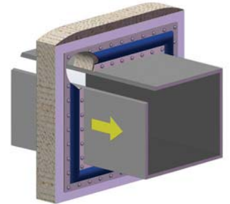
Thorburn's penetration air seal stack expansion joints are easily accessible for inspection or repair
