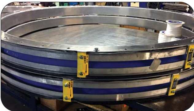
Thorburn's Flexi-Duct™ expansion joints manufactured with Aluminum 6061-T6 (SB-209) frames & backing bars to resist corrosion and reduce weight on the aluminum ducting system
