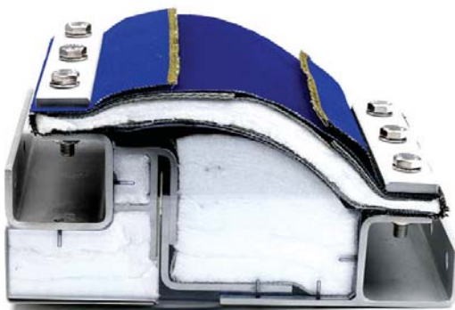
Integral flow liner
